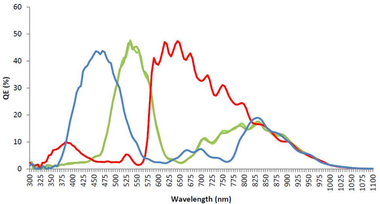
ID2MC-CL (Color)
