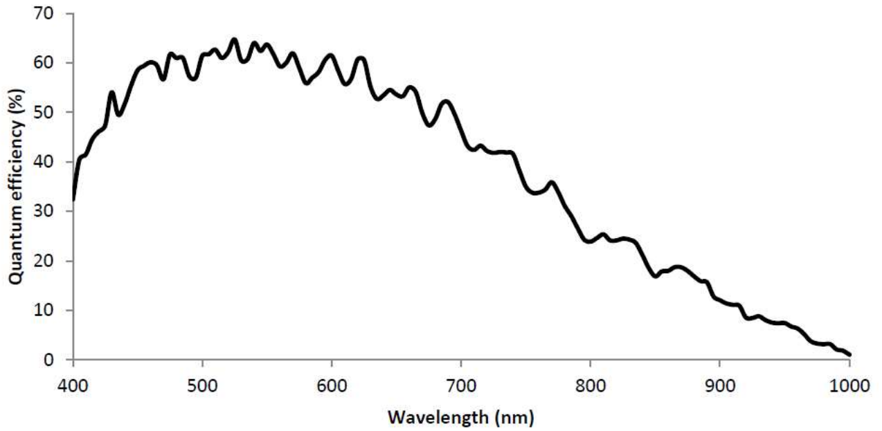
ID2MB-CL (B/W)
